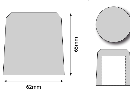
Top and Cross Section View
